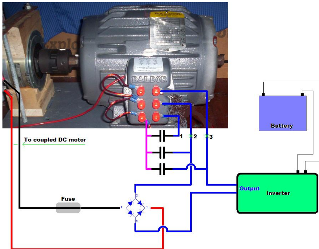
Another DC humping AC schematic
