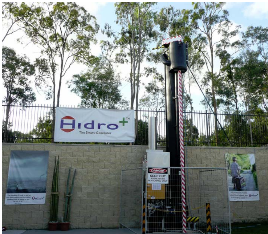
The 20 kW Hidro system evaluated by both Queensland University and Panacea
