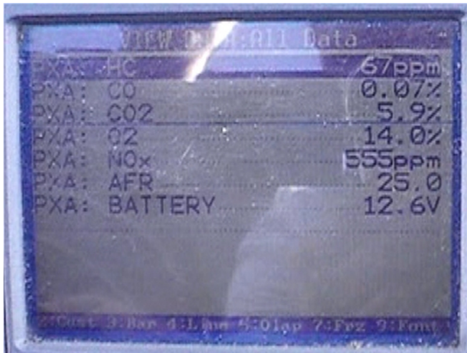
Emissions test with the SPAD activated
