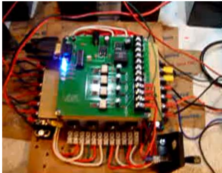
Matt Jones replicated Tesla Switch.
