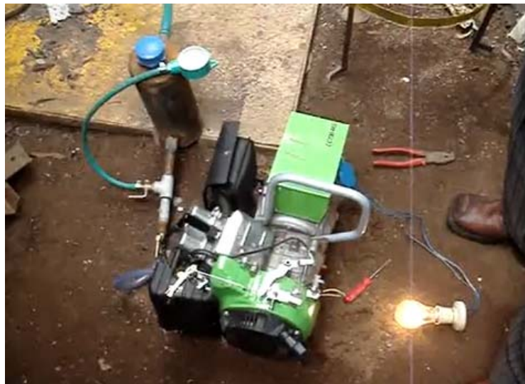
kitchen-waste-produced-biogas on our porch.
